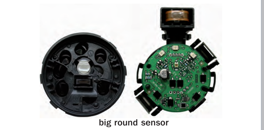
901CP big round sensor
